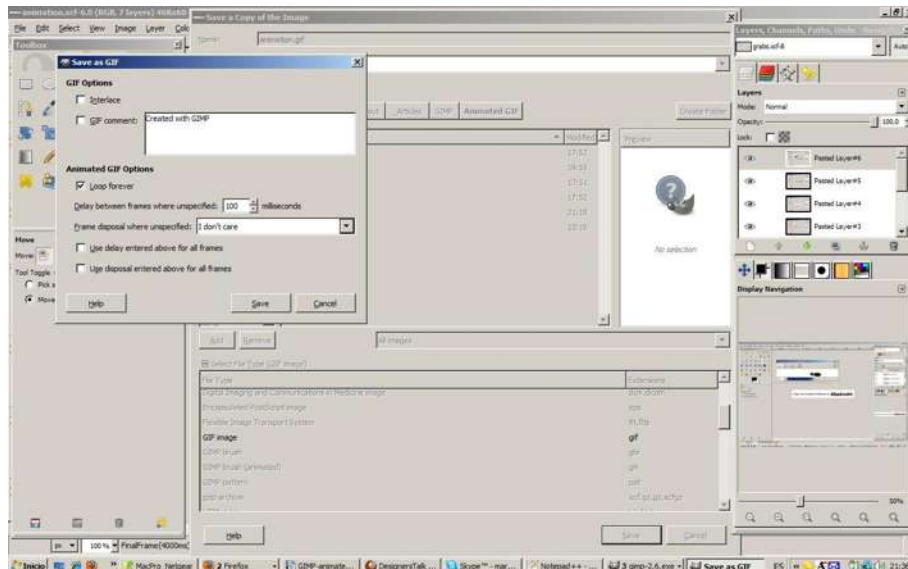
Gambar 10.6 Setting Frame 8
