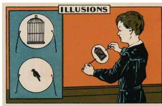
Gambar 1.6 Thaumatrope
