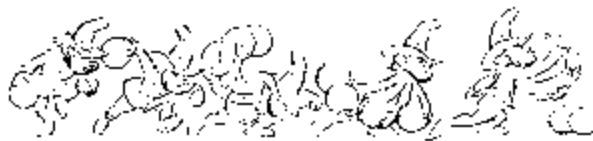
Gambar 3.3 Contoh-contoh Anticipation
