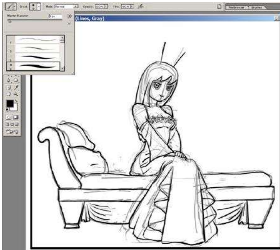
Gambar 15.2 Tracing
