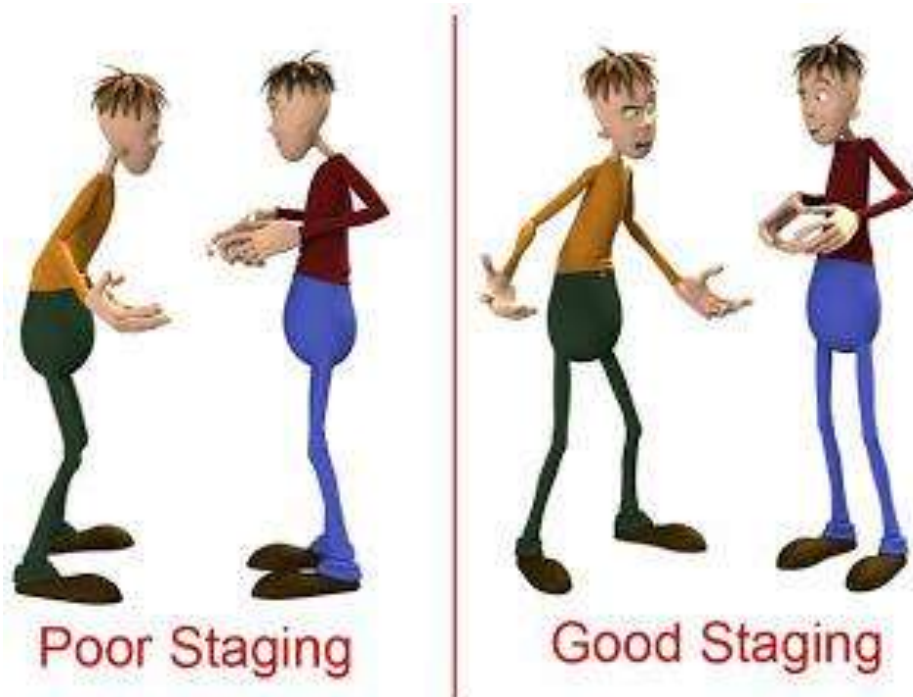
Gambar 3.6 Contoh Staging
